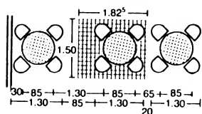
⑥ Café table arrangement
